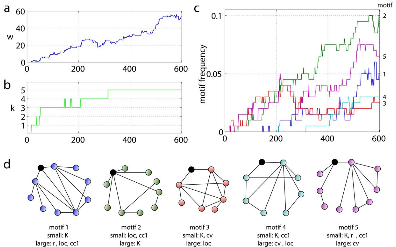
Figure 3. Single node-motifs in emerging small-world network (Fig. S2). Vertical axes in subfigures a–c correspond to number of outlier nodes w , number of single node-motifs k , and their frequencies, respectively. a Number of identified outliers w rising from 0 to 54. b Diversity of node-motifs k quickly rising during the 1st re-wiring round; less increase during 2nd round; and stable during the 3rd. c Proportions of nodes expressing identified motifs ( motif frequencies ). Nodes classified regular not shown. d Schematics of identified single node-motifs and their distinguishing characteristics.
