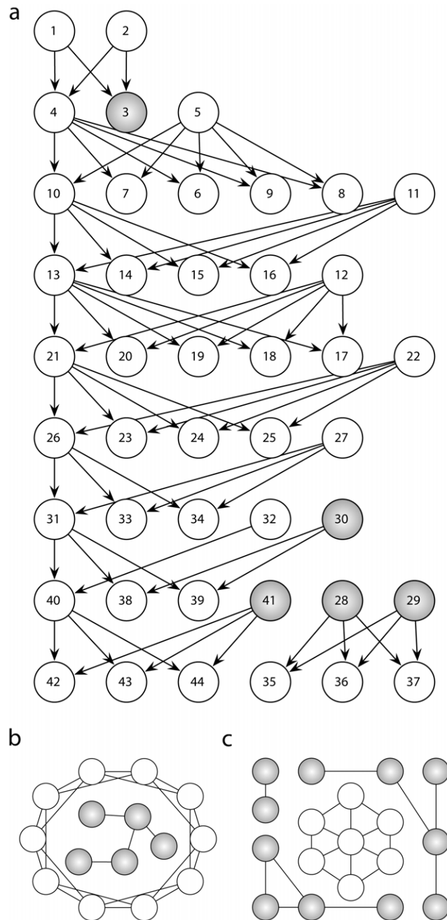
Figure 2. Network types used for testing BtA: a Network derived from The Simpsons family-tree [54]. Nodes in very regular parts of the network were identified singular (shaded grey) because of two characteristics: Their neighbours' degrees are comparatively low and show no variation (values r and c_V significantly below average). b Schematic of large regular ring lattice combined with a minor ER-random component (shaded grey). c A small regular structure (white nodes) embedded into a large random network (ER, BA, or WS model). doi:10.1371/journal.pone.0015765.g002
