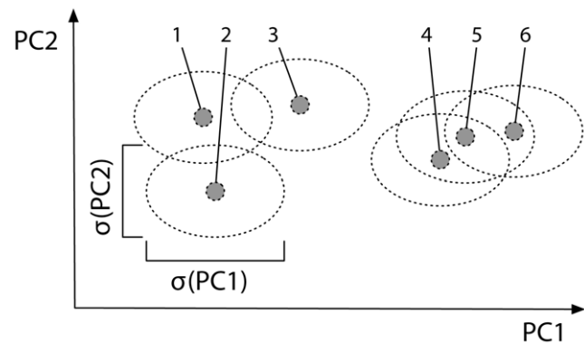
Figure 4. Example of 2 clusters (left, right) with 3 points each (1–3, 4–6). Ellipses are centred on each point with dimensions corresponding to standard deviations \sigma along PC-axes. A set of points is considered a clique , if the area of all their ellipses is connected (e.g. {1}, {1, 2}, or {1, 2, 3}; but not {2,3}). A maximal clique is called a cluster (i.e. {1,2,3} or {4,5,6}) and is used to define a distinct motif-group. doi:10.1371/journal.pone.0015765.g004
