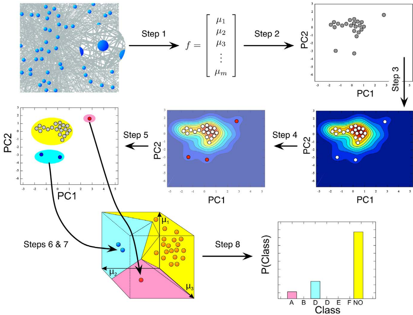
Figure 1. Analysis work-flow to identify global singular nodes from local features [41]. Step 1: Choose set of local measures to characterise network nodes [35]. Calculate local measurements for all nodes in the network ( feature vectors ). Step 2: Map each node's feature vector to lower dimensional space using principal component analysis (PCA plane) [45, Chapter 8]. Step 3: Estimate each node's probability using the Parzen window approach (PDF) [46, 47, Chapter 4.3]. Step 4: Query PDF to identify least probable nodes ( singular nodes ). Step 5: Cluster singular nodes in PCA plane using k-means ( motif groups ) [65, Chapter 20.1]. Step 6: Determine Voronoi cells for grouped nodes using a modified Mahalanobis distance ( potential motif regions ) [69]. Step 7: Join potential motif regions that are close to each other ( motif regions ). Step 8: Calculate relative frequencies of nodes falling into motif-regions (A–F) or non-motif region (NO) ( fingerprint ). doi:10.1371/journal.pone.0015765.g001
